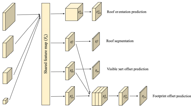
Fig. 4. Network structure of visible component prediction heads and footprint offset prediction head of our WS-MTBR-Net.
