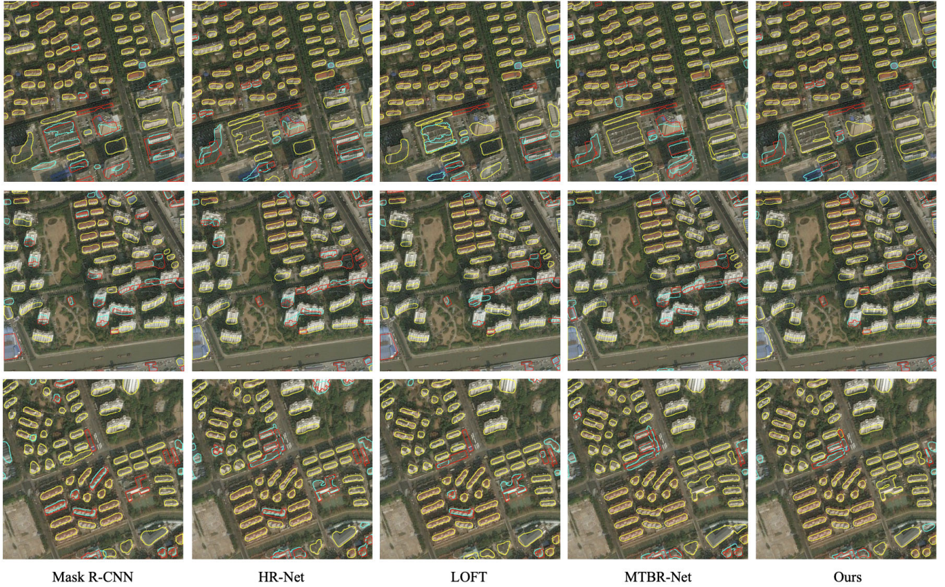
Fig. 8. Examples of building footprint segmentation results of different methods on the BONAI Shanghai test dataset. The yellow, cyan, and red polygons denote the TP, FP, and FN, respectively. Our method produces much more accurate footprint boundaries compared with other methods.
